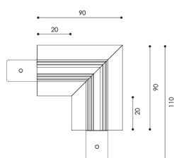
I L-90°hoek (trimless)
